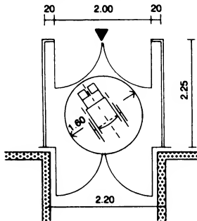
③ Porch with two-leaf door
